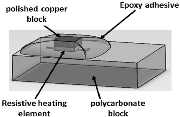
Fig. 1. Design of the test heater for the boiling experiment.
