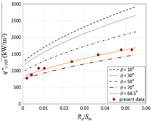
Fig. 13. Trend of Eq. (26) at different contact angles of 10^\circ , 30^\circ , 50^\circ , and 70^\circ and comparison with the measured data at the contact angle of 64.5^\circ .
