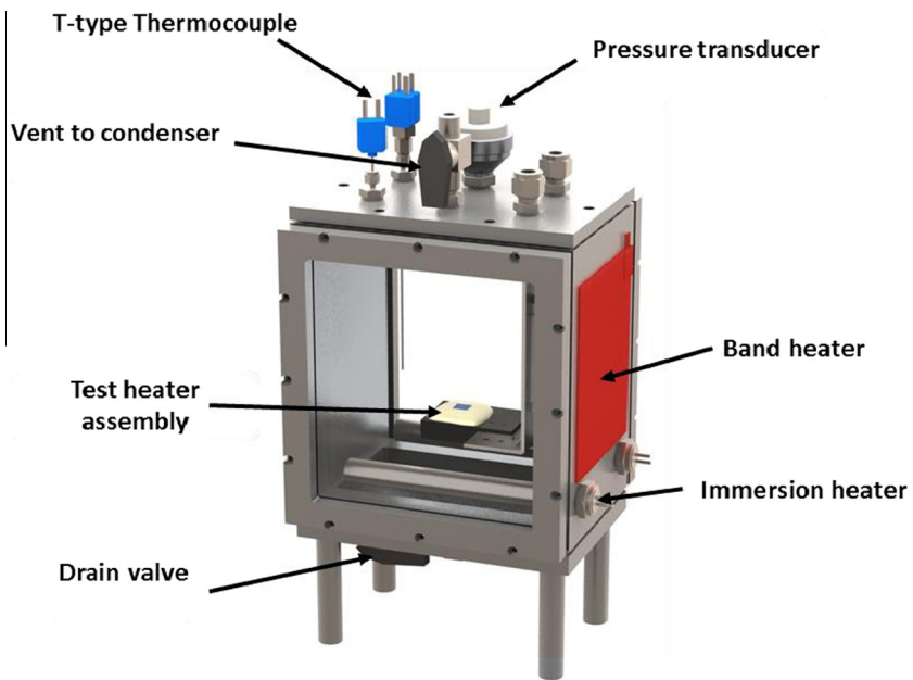
Fig. 2. Detailed drawing of the boiling test chamber.
