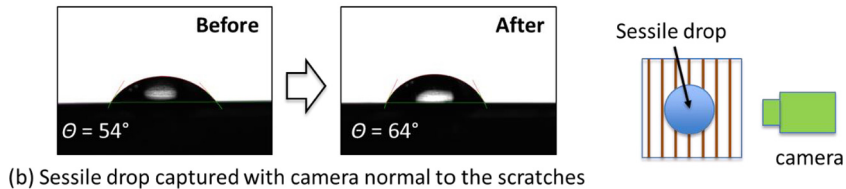
Fig. 4. Static contact angles at two directions: (a) parallel to the scratches, (b) normal to the scratches ( R_a = 0.169 \mu\text{m} , 600 grit #1).
