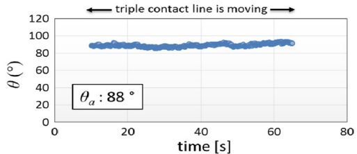
(a) Advancing contact angle (before boiling, parallel)
