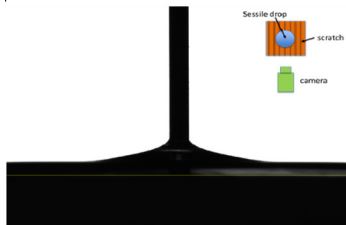
(b) Receding contact angle (before boiling, parallel)
