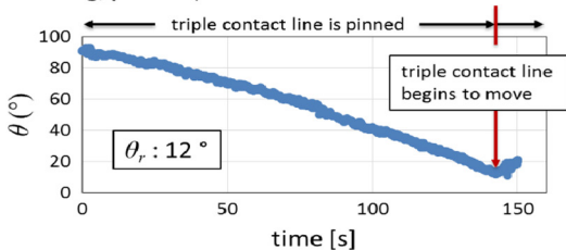
(b) Receding contact angle (before boiling, parallel)
