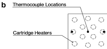
Fig. 1. (a) Schematic diagram of the experimental facility with relevant components indicated and (b) top view of the test block.
