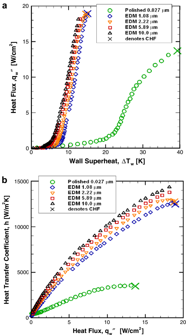
Fig. 3. Boiling curves for FC-77 on five surfaces of varying roughness: (a) heat flux versus wall superheat and (b) heat transfer coefficient versus heat flux, after (Jones et al., 2009).
