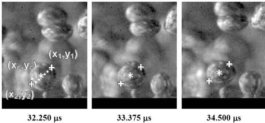
Fig. 6. Illustration of bubble measurement technique showing diametrical points logged (+) and the calculated centroid location (*) of a bubble produced on the polished surface at 2.06 W/cm 2 .
