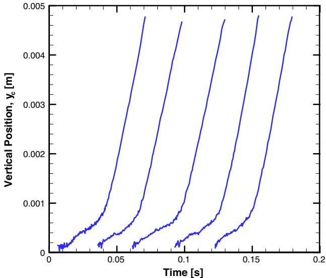
Fig. 7. Time history of the vertical position of five consecutive bubbles originating from a single active nucleation site on the polished surface at 2.06 \text{ W/cm}^2 .
