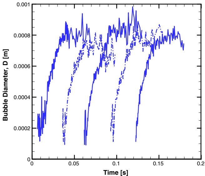
Fig. 9. Growth of five consecutive bubbles originating from a single active nucleation site on the polished surface at 2.06 \text{ W/cm}^2 .
