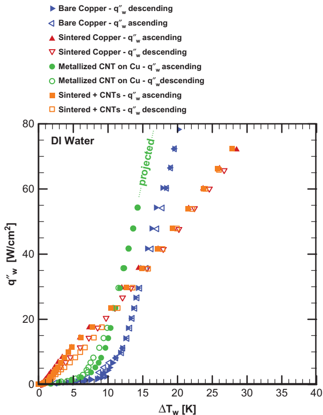
Figure 4 DI water pool boiling curves for the enhanced surfaces and the plain surface (color figure available online).
