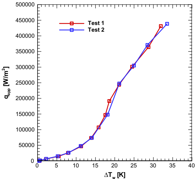
Fig. 6. Apparent boiling curves (heat flux uncorrected) measured by the 400 \mu m \times 25 \text{ mm} ITO heater/sensor test strip of surface 5. Good repeatability was obtained between tests.
