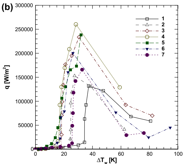
Fig. 9. Boiling curves for the seven surfaces tested: (a) apparent (uncorrected) heat flux values, and (b) heat flux values corrected by the method of Section 5.1.
