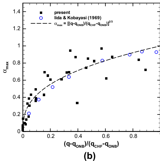
Fig. 11. (a) Approximate void fraction distribution above surface 3 at three different heat fluxes. (b) Maximum void fraction can be correlated with normalized nucleate boiling heat flux. The present data (FC-72) compare well with those of Iida and Kobayasi [57] (water).
