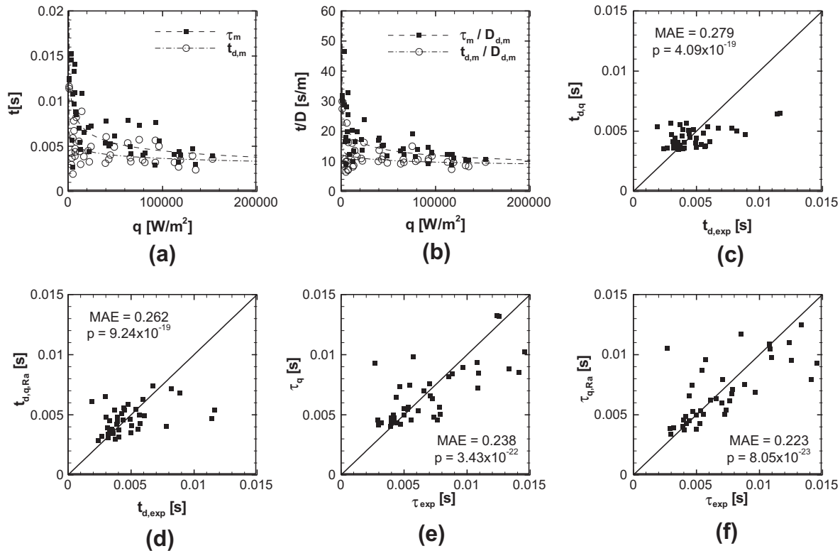
Fig. 7. Comparisons of experimental data and predicted values for power curve fits between mean bubble growth period t_d or total ebullition period \tau and heat flux, and departure diameter.
