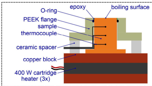
Figure 2. Experimental setup ( top ), heating block and sample assembly ( bottom left ) and sample dimensions including thermocouple locations ( bottom right ).
