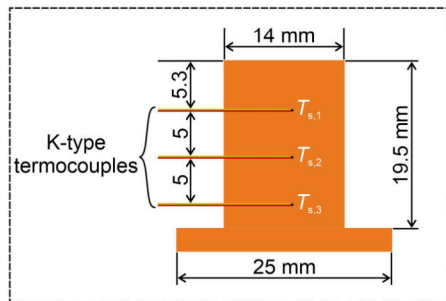
Figure 2. Experimental setup ( top ), heating block and sample assembly ( bottom left ) and sample dimensions including thermocouple locations ( bottom right ).
