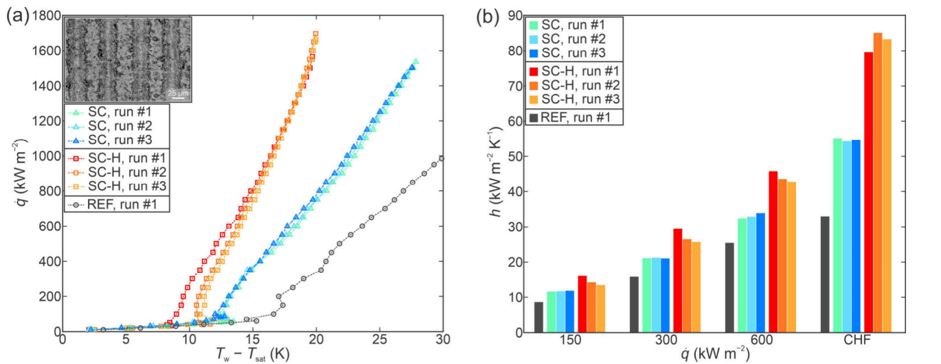
Figure 5. Boiling performance of the shallow channel sample (SC) evaluated through (a) boiling curves and (b) heat transfer coefficients at selected heat fluxes.
