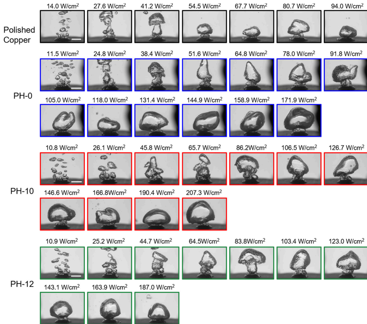
Fig. 11. Representative boiling images at different heat fluxes for polished copper and copper foams deposited at pH 0, pH 10, and pH 12. The scale bar represents 10 mm.
