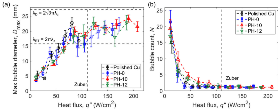
Fig. 12. Bubble dynamics analysis during pool boiling showing (a) the maximum bubble diameter and (b) bubble count at different heat fluxes for water boiling on polished copper and copper foams deposited at pH 0, pH 10, and pH 12.
