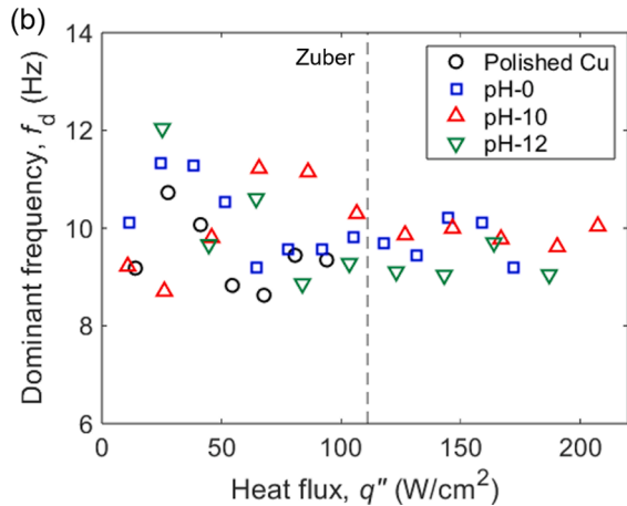
Fig. 14. Spectral analysis of vapor fraction during boiling showing (a) power of the vapor fraction spectral as a function of heat flux and (b) dominant frequency as a function of heat flux.
