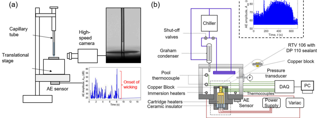
Fig. 4. Schematic diagrams of (a) the surface wickability testing facility with the inset showing a representative optical image and acoustic signals and (b) the pool boiling test facility with the inset showing representative acoustic signals.
