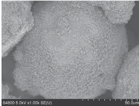
Figure 1 SEM images of boiling surfaces fabricated for this work: (a) porous layer formed of sintered copper spheres, (b) Cu-metallized MWCNT array, and (c) sintered Cu spheres with metallized CNT array grown after sintering.
