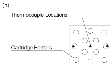
Figure 2 (a) Schematic diagram of the experimental facility with relevant components indicated and (b) top view of the test block (adapted from McHale and Garimella [26]).
