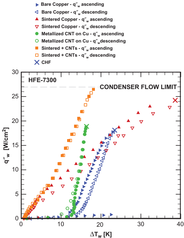
Figure 3 HFE-7300 pool boiling curves for the enhanced surfaces and the plain surface (color figure available online).
