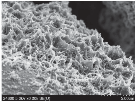
Figure 6 SEM images of the sintered boiling surface after pool boiling tests and desoldering.
