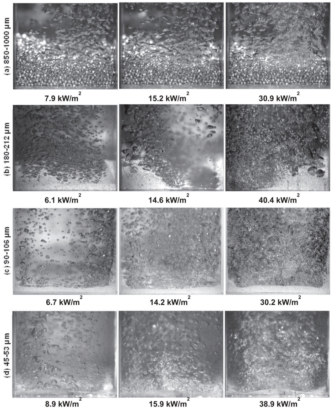
Fig. 5. Images taken from high-speed visualization at 2000 fps for (a) 850–1000 \mu\text{m} , (b) 180–212 \mu\text{m} , (c) 90–106 \mu\text{m} , and (d) 45–53 \mu\text{m} free particle diameters at similar heat fluxes throughout the boiling curve (see Supplementary Video Data ).
