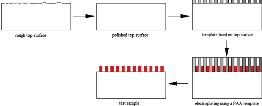
Fig. 3. The synthesis process of copper nanowire array on the top surface of copper block.
