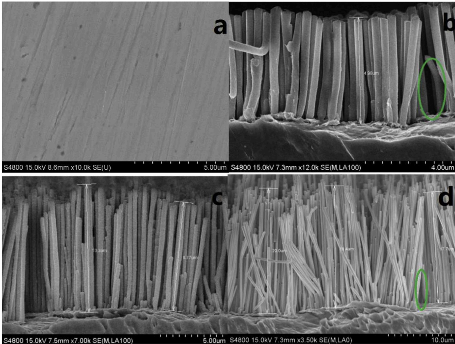
Fig. 5. SEM photograph of a) smooth surface (top view), b) 5 \mu\text{m} NWs, c) 10 \mu\text{m} NWs, and d) 20 \mu\text{m} NWs.
