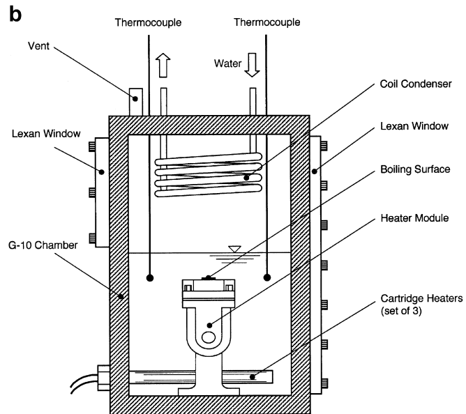
Fig. 2. Schematics of (a) heater module assembly and (b) boiling facility.
