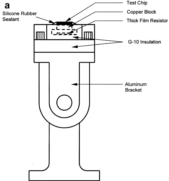
Fig. 2. Schematics of (a) heater module assembly and (b) boiling facility.
