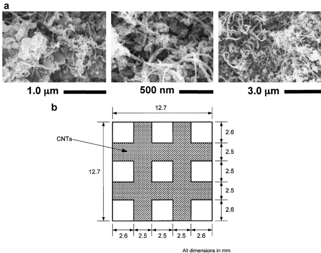
Fig. 4. (a) SEM images and (b) CNT layout on 'grid'-patterned surface.
