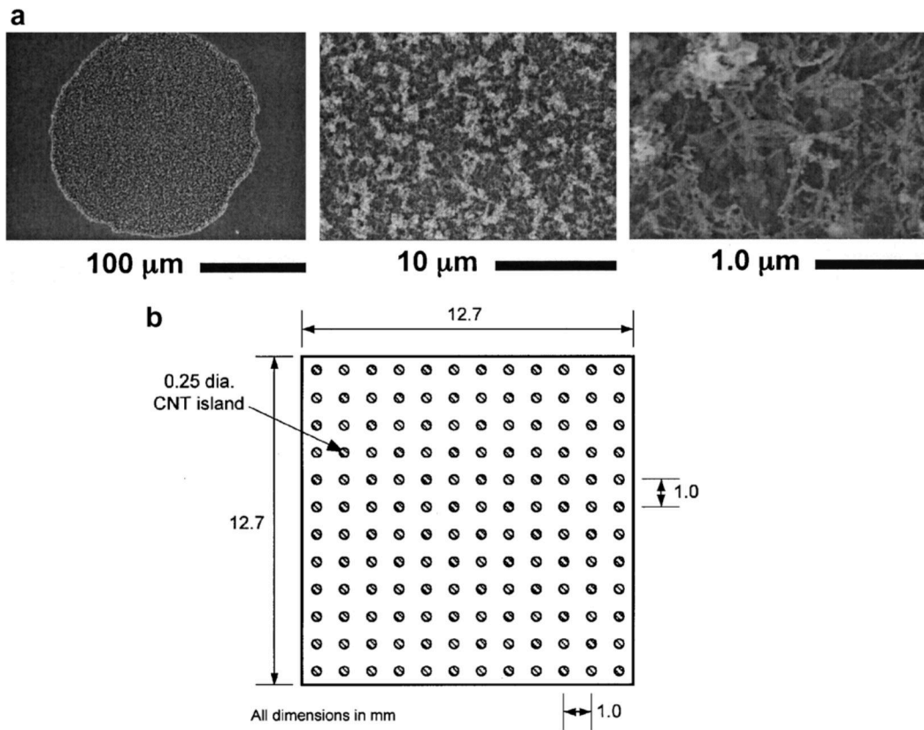
Fig. 5. (a) SEM images and (b) CNT layout on 'island'-patterned surface.
