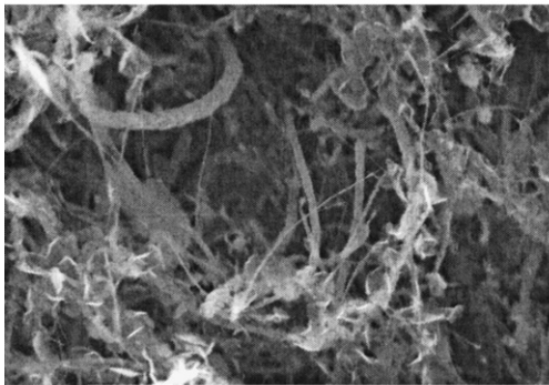
Fig. 6. SEM images of CNT-coated flat copper surface.
