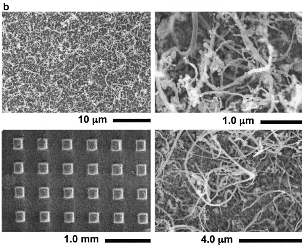
Fig. 7. (a) Dimensions of copper microstud surface. (b) SEM images of CNT-coated copper microstud surface.
