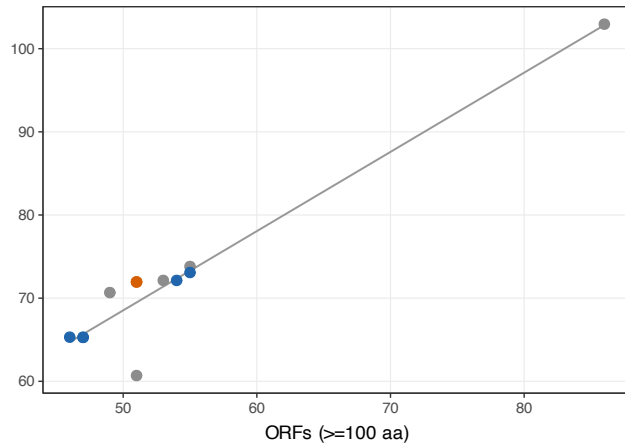
b and ORF count more so ( r = +0.96 )
