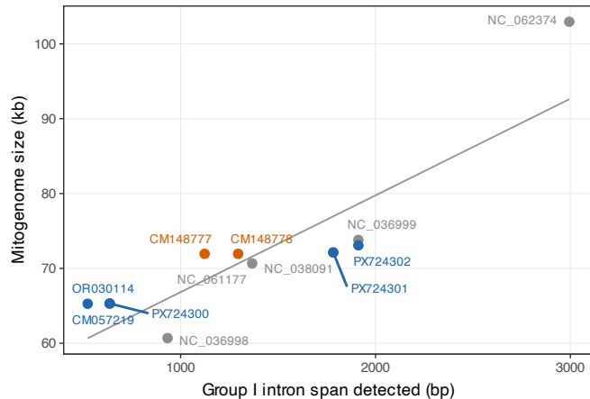
a Intron content tracks genome size ( r = +0.87 )
