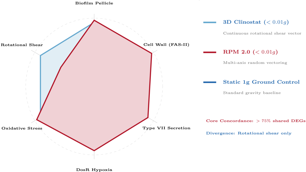
a Biological Response Trajectory Radar Across Simulation Modalities
