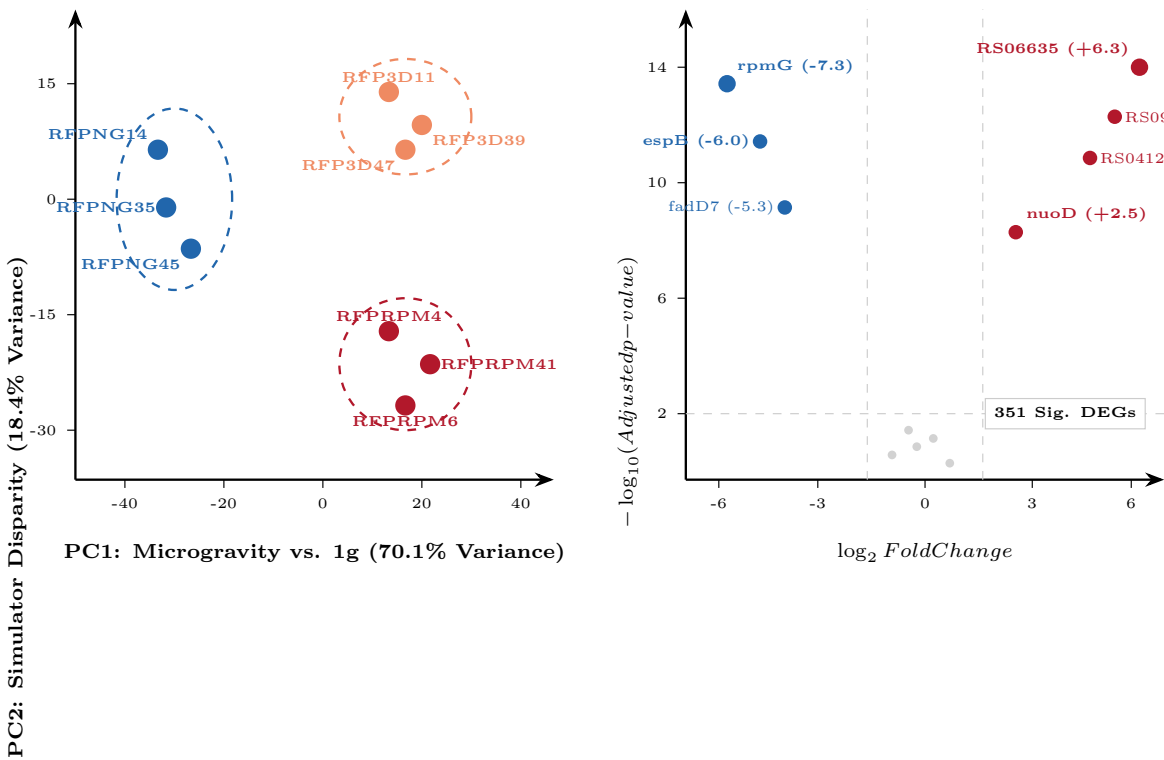
a Transcriptomic Principal Component Analysis 3D Clinostat vs. Static 1g (351 DEGs)
