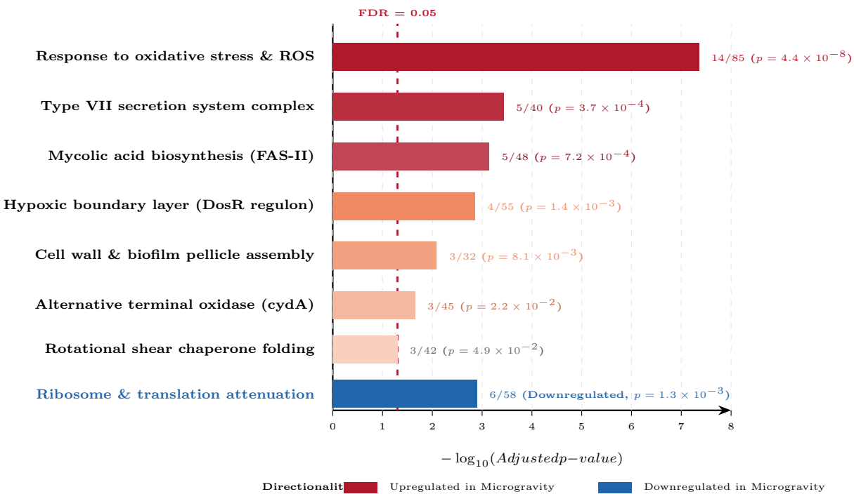
a Enriched GOSlim Functional Pathways in Simulated Microgravity
