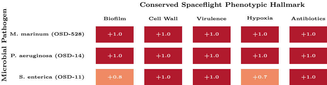
b Cross-Species Spaceflight Adaptation Concordance
