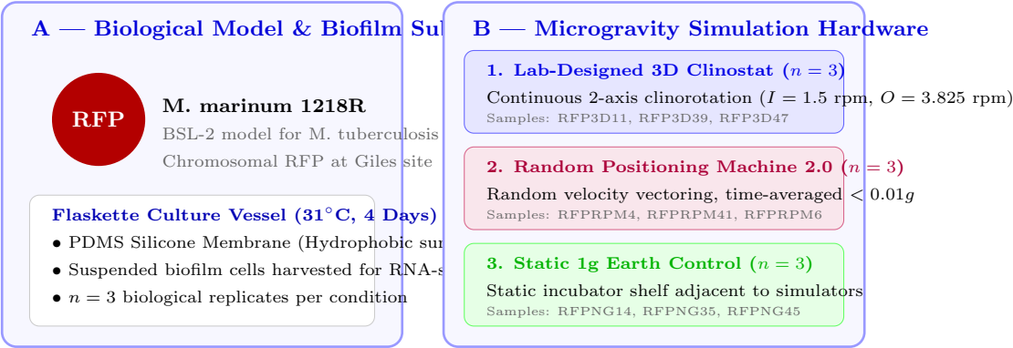
Figure 1 — Systems Architecture and Experimental Framework of NASA OSDR OSD-528 Comparative simulated microgravity modalities (3D Clinostat vs. RPM 2.0 vs. 1g Static) in Mycobacterium marinum (Clary et al., 2022)
