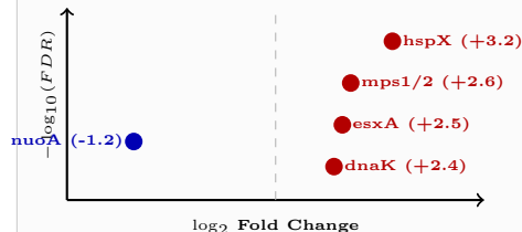
B — Volcano: 3D Clinostat vs. Static 1g (105 DEGs)
