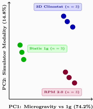
A — Principal Component Analysis
