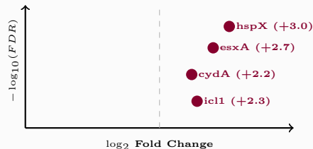
C — Volcano: RPM 2.0 vs. Static 1g (162 DEGs)
