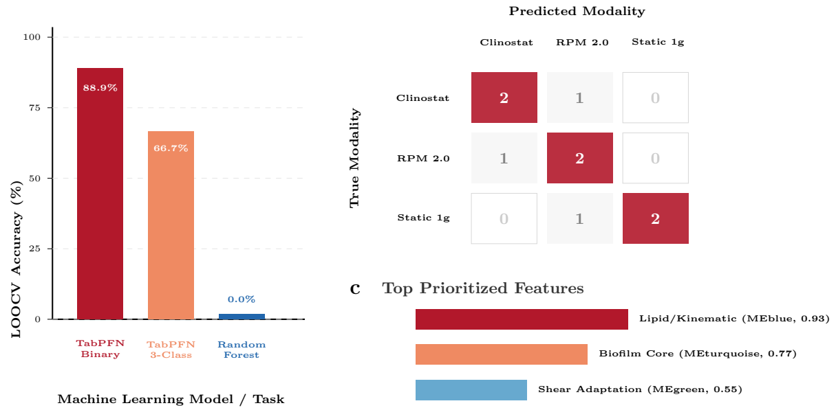
a Leave-One-Out Cross-Validation (LOOCV) TabPFN 3-Class Confusion Matrix (LOOCV)
