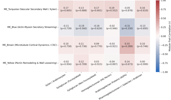
WGCNA Module-Glycan Trait Relationships Co-expression Transcript Modules Correlated with OSD-615 Wall Epitopes
