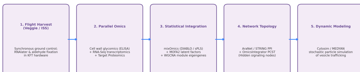
Figure 10: Comprehensive Mass Spectrometry and Glycome Profiling Workflows. A , Advanced mass spectrometry workflow for mapping O -GlcNAcylation sites on cytoskeletal motor complexes (ETHcD LC-MS/MS). B , CCRC sequential chemical fractionation and high-throughput glycome ELISA workflow (OSD-615). C , Proposed multi-omics systems integration framework.
