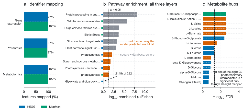
Fig. 6 Pathway integration across all three layers. In b a square marks each pathway's database, in the colours of a : KEGG's Photosynthesis and MapMan's photosynthesis are different maps that differ only in capitalisation, and both are significant.
