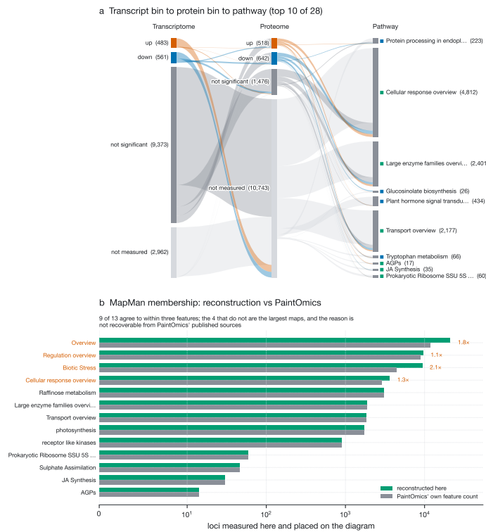
Fig. S1 Where the loci go, and how far the MapMan half of the diagram can be trusted. a , Each locus in at least one of the 28 non-whole-ontology significant pathways is placed in one transcript bin and one protein bin, and then into the pathways it belongs to. Ribbon width is a locus count. The transcript and protein columns conserve loci exactly; the pathway column counts memberships , so a locus in more than one pathway is counted more than once. The pathway column draws the ten most significant; a square gives each pathway's database in the colours of Fig. 6a. Three whole-ontology MapMan diagrams are excluded — Overview lists all 36 top-level bins and so covers 99.8% of measured loci, and Regulation overview and Biotic Stress cover 45% and 44%; the next largest covers 17%. A map holding nearly every measured locus cannot say where anything goes, because its ribbons reproduce the marginal distribution. b , PaintOmics reports enrichment but not the gene lists behind it, and MapMan has no equivalent of the KEGG REST API, so MapMan membership is reconstructed from GoMapMan's Araport11 gene-to-bin mapping and the MapMan diagram layouts, by PaintOmics' own inclusion rules. Reconstructed membership is compared against the feature count PaintOmics itself reported for each diagram (log scale). Nine of the thirteen agree to within three features. The four that do not are the largest maps, are marked in vermilion with the ratio between the two counts, and the reason for the difference is not recoverable from PaintOmics' published sources; both counts are reported rather than one.
