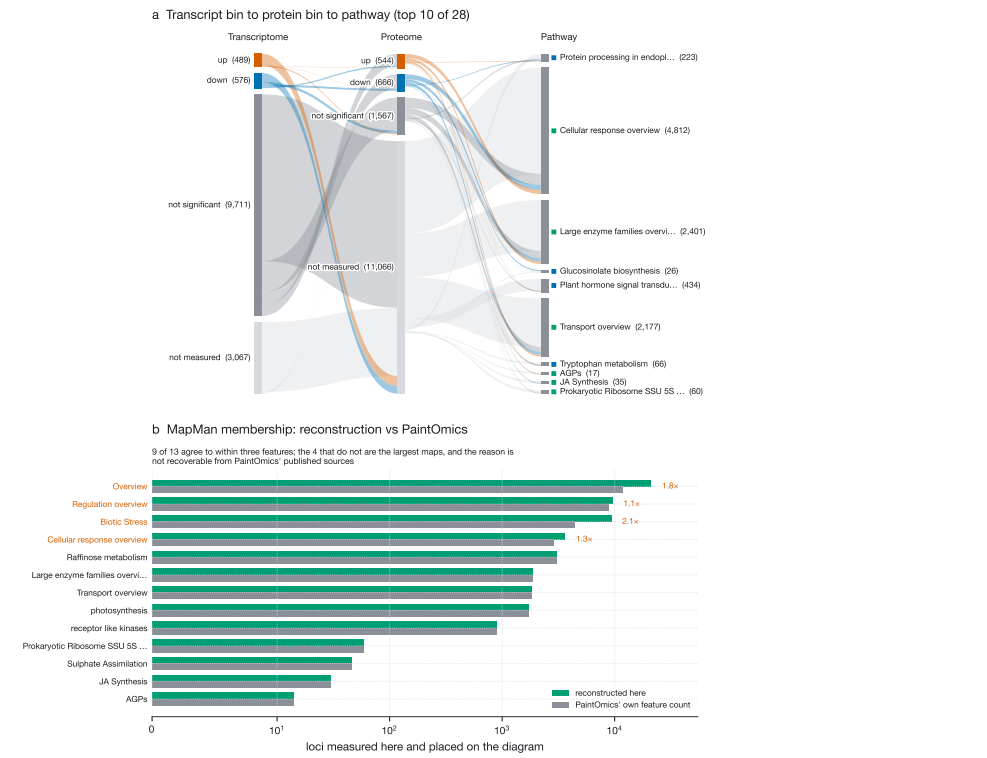
Fig. S1 Locus-level multi-omics flow and MapMan ontology reconstruction. a, Each locus in at least one of the 28 non-whole-ontology significant pathways is placed in one transcript bin and one protein bin, and then into the pathways it belongs to. Ribbon width is proportional to locus count. The pathway column draws the ten most significant pathways; a square gives each pathway's database in the colours of Fig. 6a. b, Reconstructed MapMan diagram membership compared against the feature count PaintOmics reported for each diagram (log scale). Nine of the thirteen diagrams agree to within three features.
