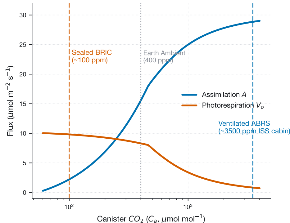
A. FvCB Photosynthesis & Photorespiration Operating Range
