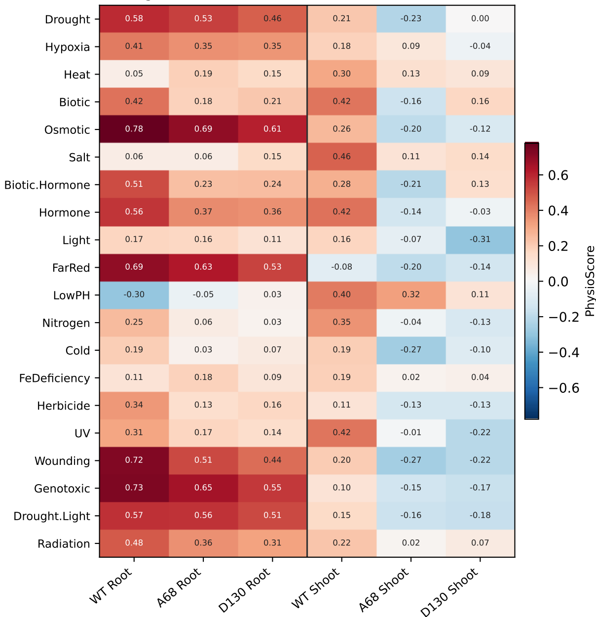
Fig 6. PhysioSpace stress-pattern decoding (Flight–Ground; bounded statistic; roots \gg shoots)
