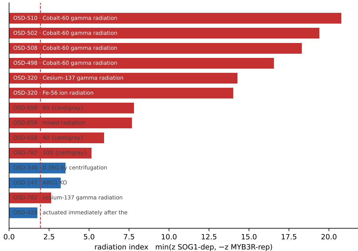
Top 14 contrasts (dashed = threshold 1.96)
