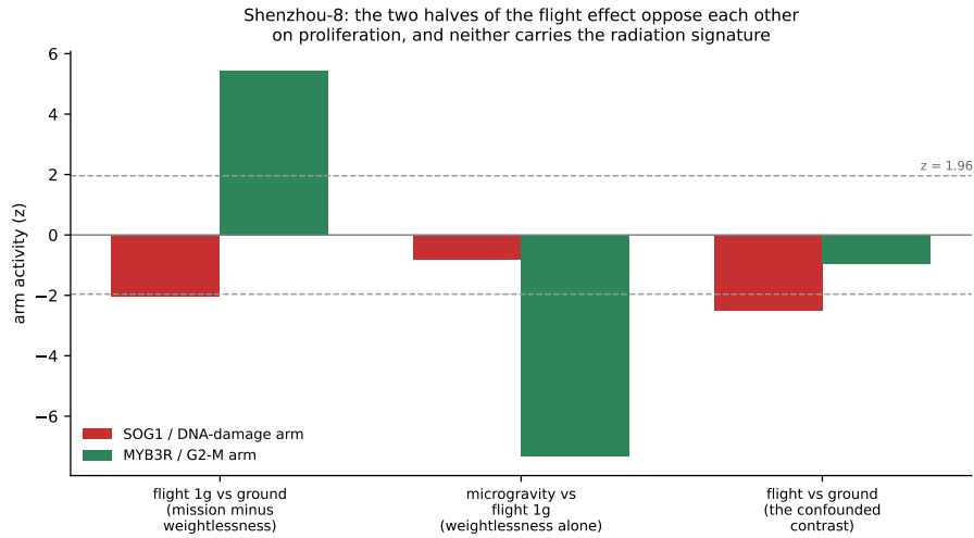
Figure 13: The Shenzhou-8 in-flight 1 g control splits the flight effect into a non-microgravity term and a microgravity term. Neither carries the radiation signature, at a mission dose far below the assay’s floor. The MYB3R/G2-M arm moves in opposite directions in the two terms and nearly cancels in the confounded flight-versus-ground contrast.
