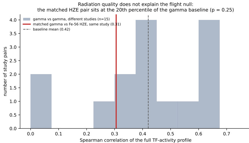
Figure 12: Radiation quality tested against the flight null. The matched gamma-versus-HZE comparison within OSD-320 falls inside the distribution of gamma-versus-gamma correlations between different studies, not below it.
