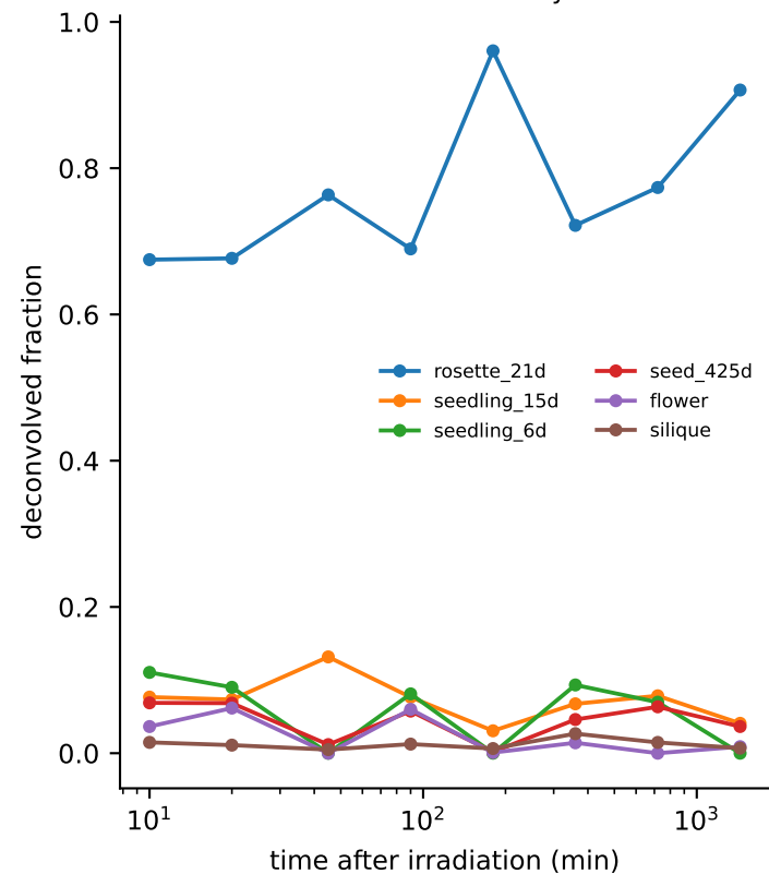
Per-timepoint fractions are unstable at both resolutions — not dynamics
