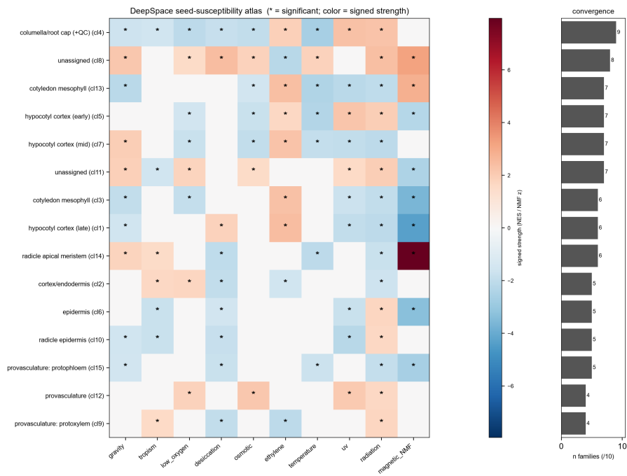
Fig 5 (HEADLINE). DeepSpace seed-susceptibility atlas: germinating-seed cell type x stressor family + multi-stressor convergence (radicle tip = top hotspot).
