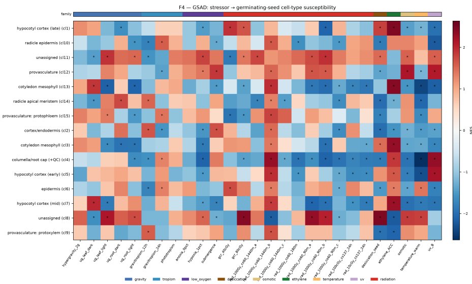
Figure 4. GSAD — stressor → germinating-seed cell-type susceptibility.
